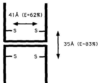
Fig. 4. Schematic representation of the location of the four Cys-949 residues in an \alpha_2M tetramer based upon measurements made here and previously [1]. The distances given are for separations between the fluorophores attached to the cysteine residues, and are based on R(2/3) values. Efficiencies of fluorescence energy transfer are given in parentheses.
