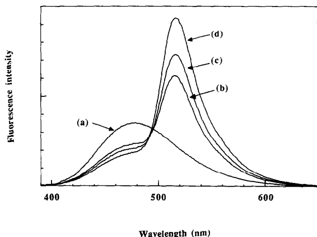
Fig. 3. Fluorescence emission spectra of labeled I-form \alpha_2M . (a) I-form \alpha_2M with dansyl label attached to one cysteine and the other cysteine blocked with iodoacetamide; (b) I-form \alpha_2M with 1.0 dansyl labels and 0.51 fluorescein labels; (c) I-form \alpha_2M with 1.0 dansyl label and 0.63 fluorescein labels; (d) I-form \alpha_2M with 1.0 dansyl label and 0.83 fluorescein labels. Spectra were recorded at equal concentrations of \alpha_2M (1.0 \mu M ) and identical spectrometer settings. All species have identical amounts and distributions of dansyl label, since they all derived from the same labeling reaction with 1,5-I-AEDANS.
